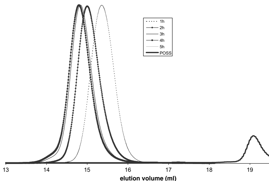
Fig. 4. Size exclusion chromatograms of POSS–PLA nanohybrids (effect of reaction time, see Table 1).
