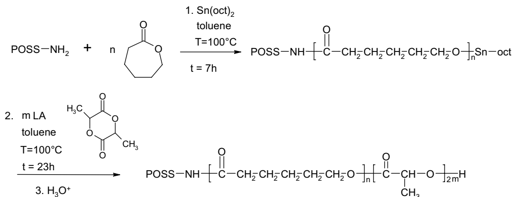
Scheme 1. Synthesis of POSS-P(CL-b-LA) block copolymer.
