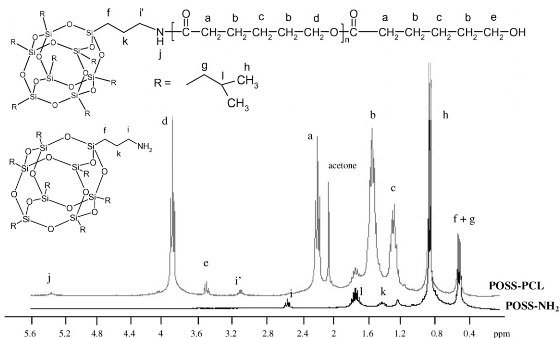
Fig. 1. 1 H NMR spectrum of the POSS–NH 2 and a POSS–PCL nanohybrid in CDCl 3 (entry 2, Table 1).
