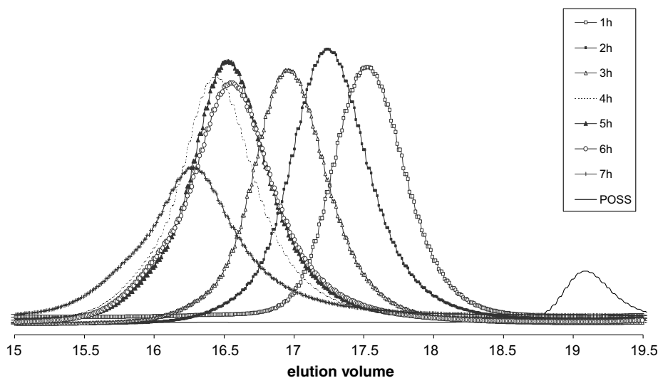
Fig. 3. Size exclusion chromatograms of POSS-PCL nanohybrids (effect of reaction time, see Table 1).
