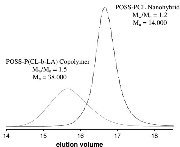
Fig. 7. SEC traces of POSS-PCL nanohybrid and POSS-P(CL-b-LA) block copolymer (see Table 2).
