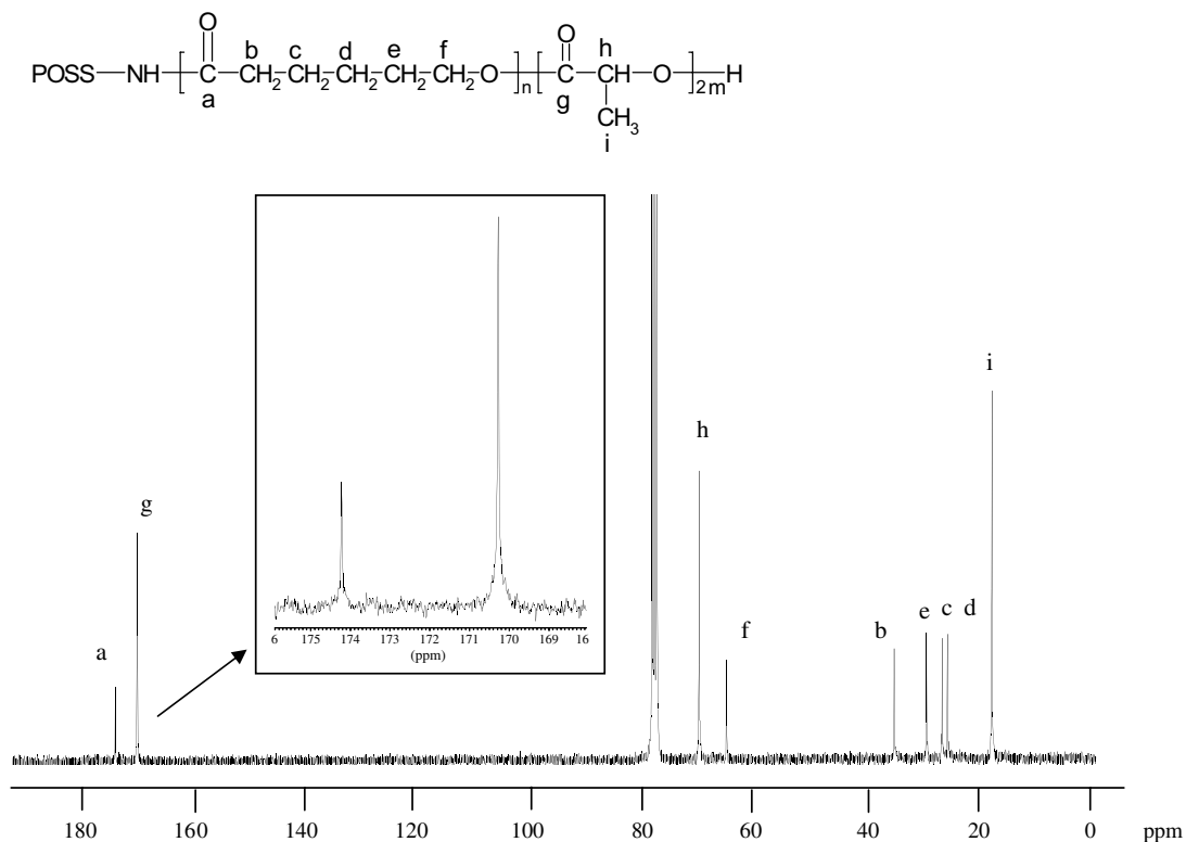
Fig. 9. 13 C NMR spectrum of POSS-P(CL-b-LA) block copolymer in CDCl 3 .
